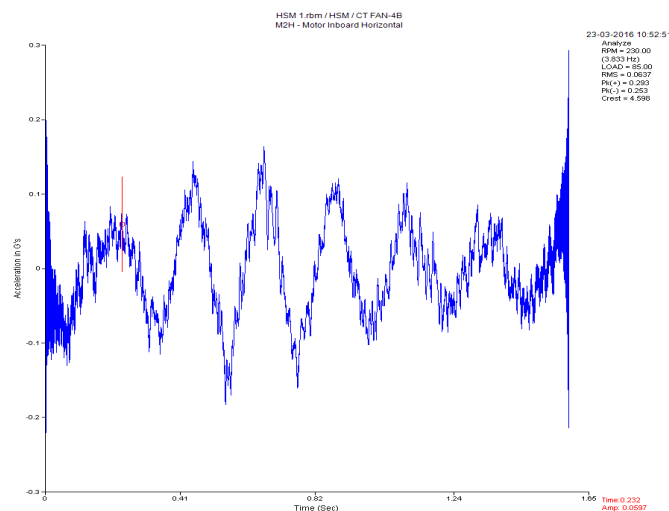
Fig.4 Acceleration Vs Time Vibration spectrum of ROT Cooling Tower FAN-B
