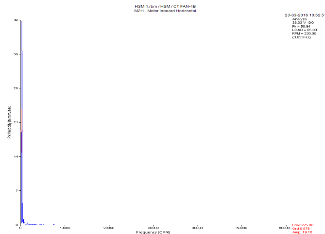
Fig.5 Amplitude Vs Frequency Vibration spectrum of ROT Cooling Tower FAN-B
