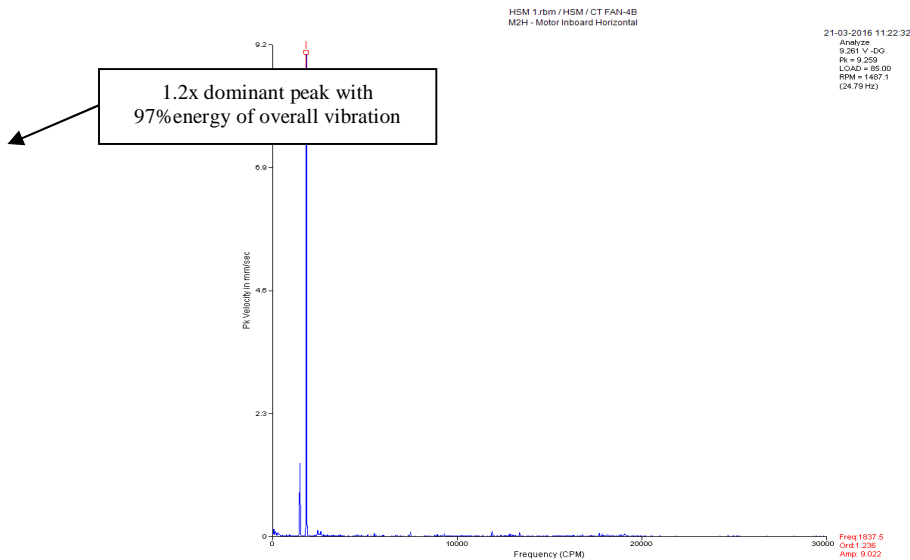
Fig.3 Vibration spectrum of ROT Cooling Tower FAN-B
