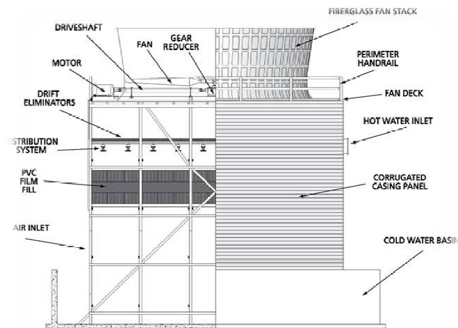
Fig.2 Structure to indicate the cooling tower fan
